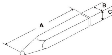
Punch Size – length and square section measured using the above diagram and below dimensions
