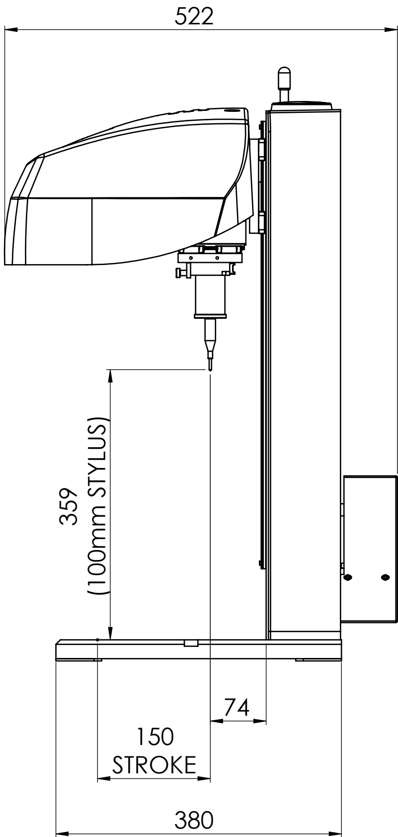
SIDE VIEW
