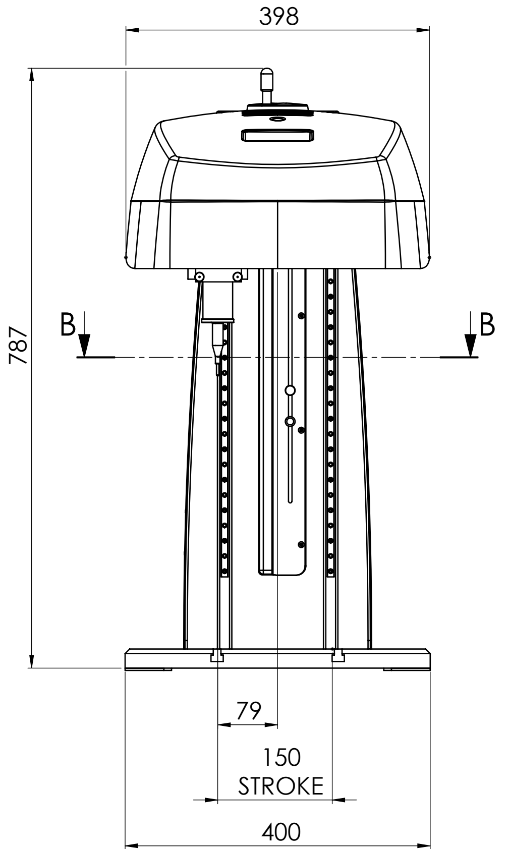
FRONT VIEW
